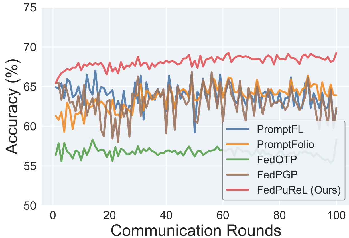
Global Model
