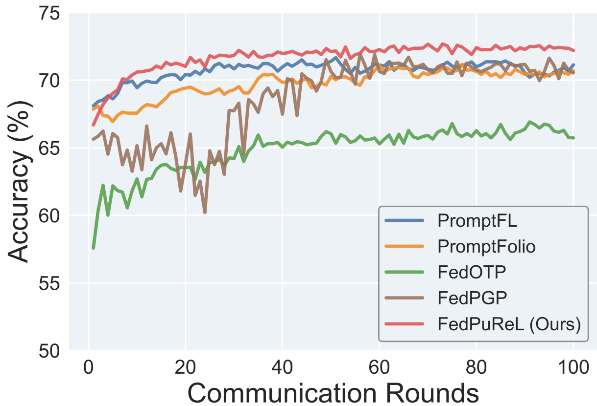
Personalized Model
