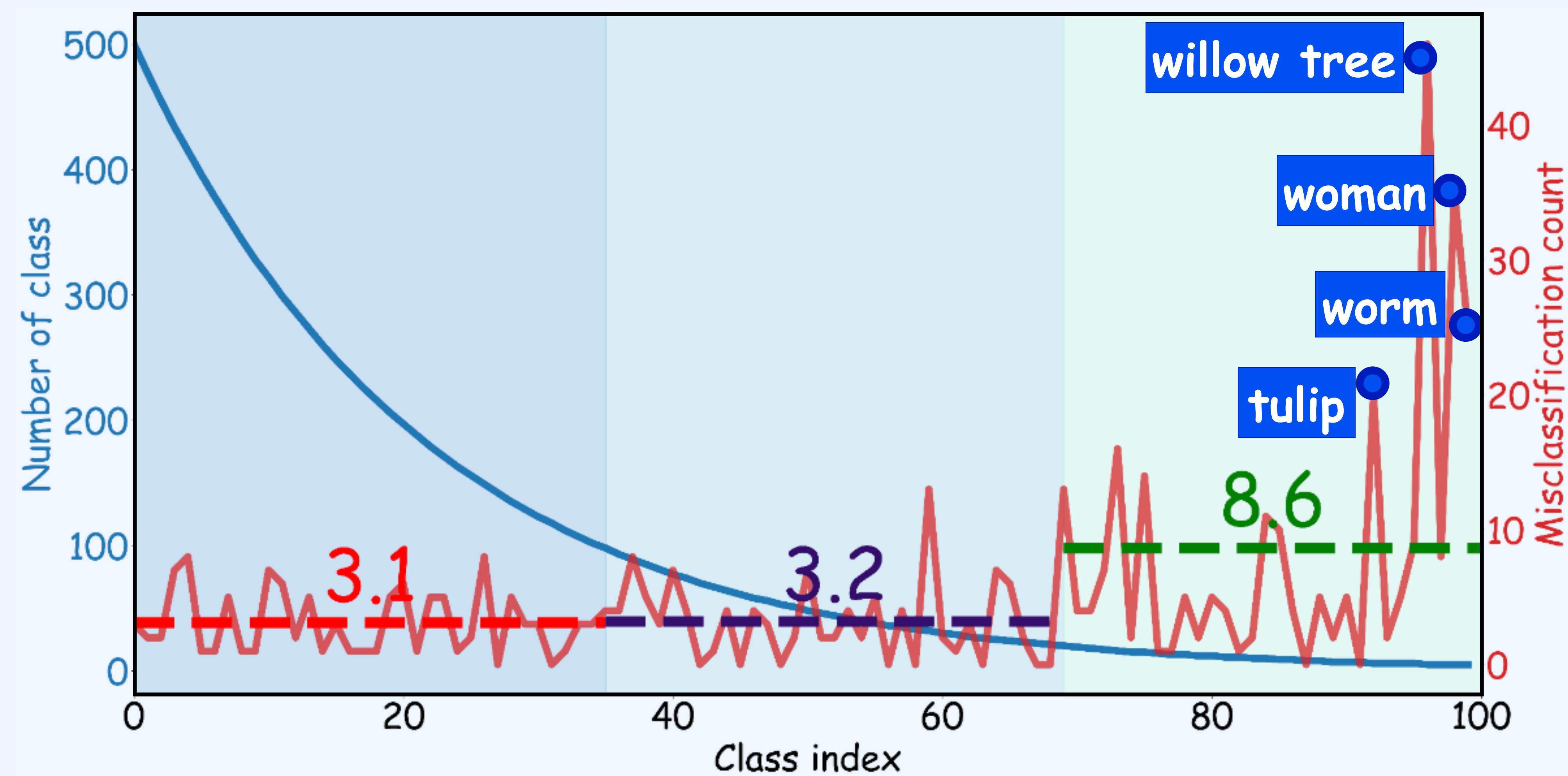
(a) New bias phenomenon
