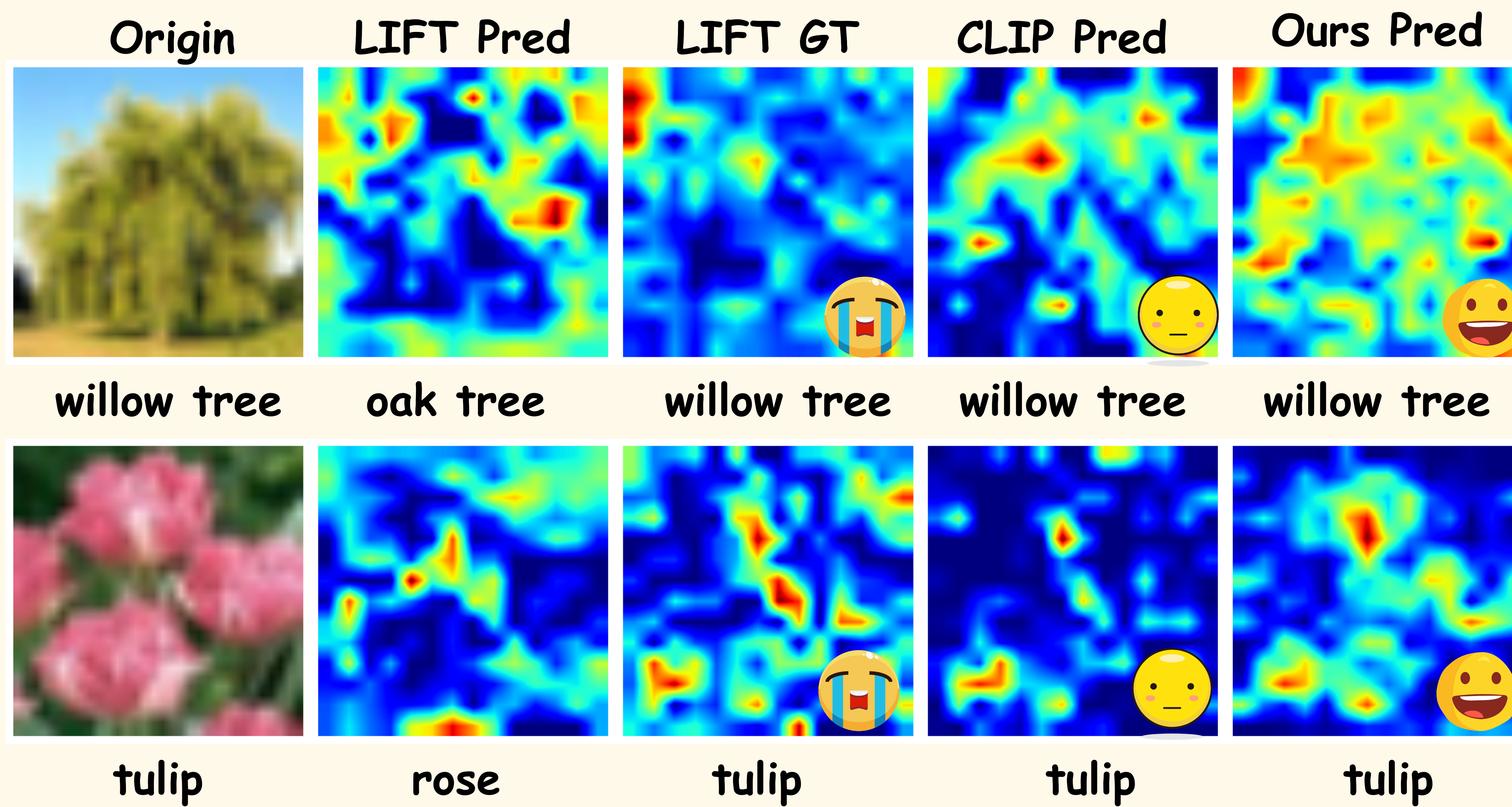
(c) Grad-CAM shown on different methods
