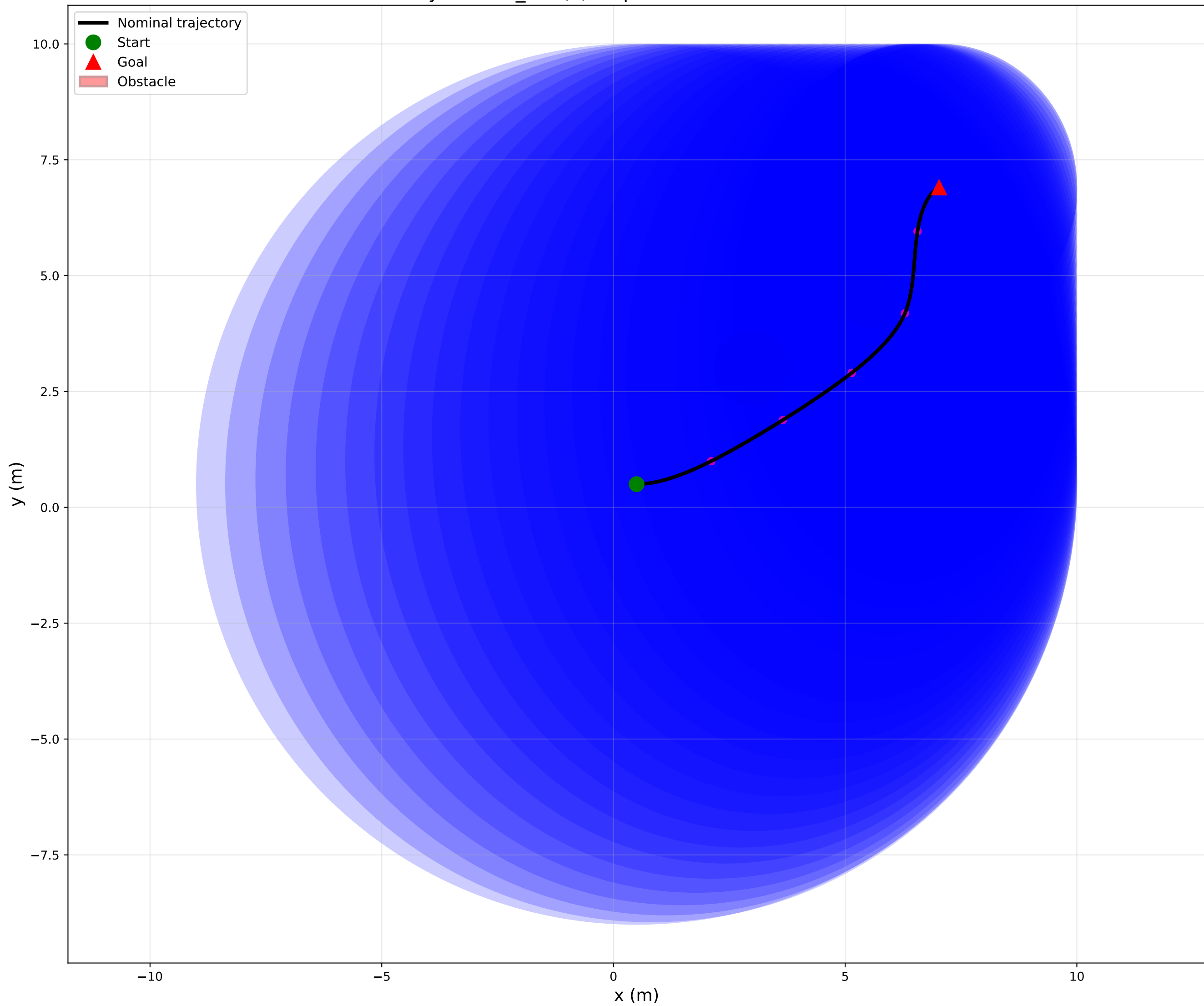
Feasibility Tube: P_{\min}(k) Ellipsoids with Obstacle Avoidance
