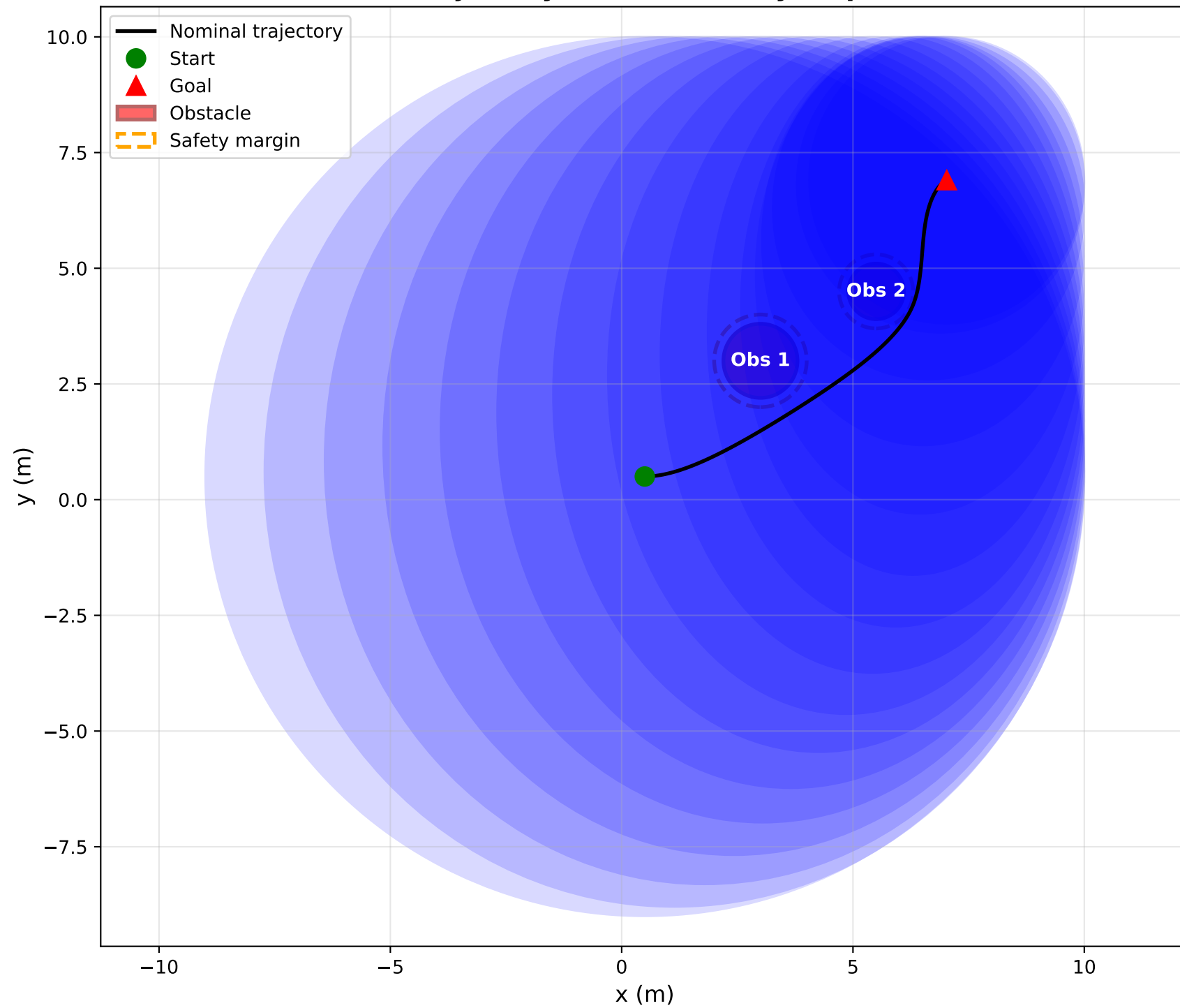
Full Trajectory with Feasibility Ellipsoids
