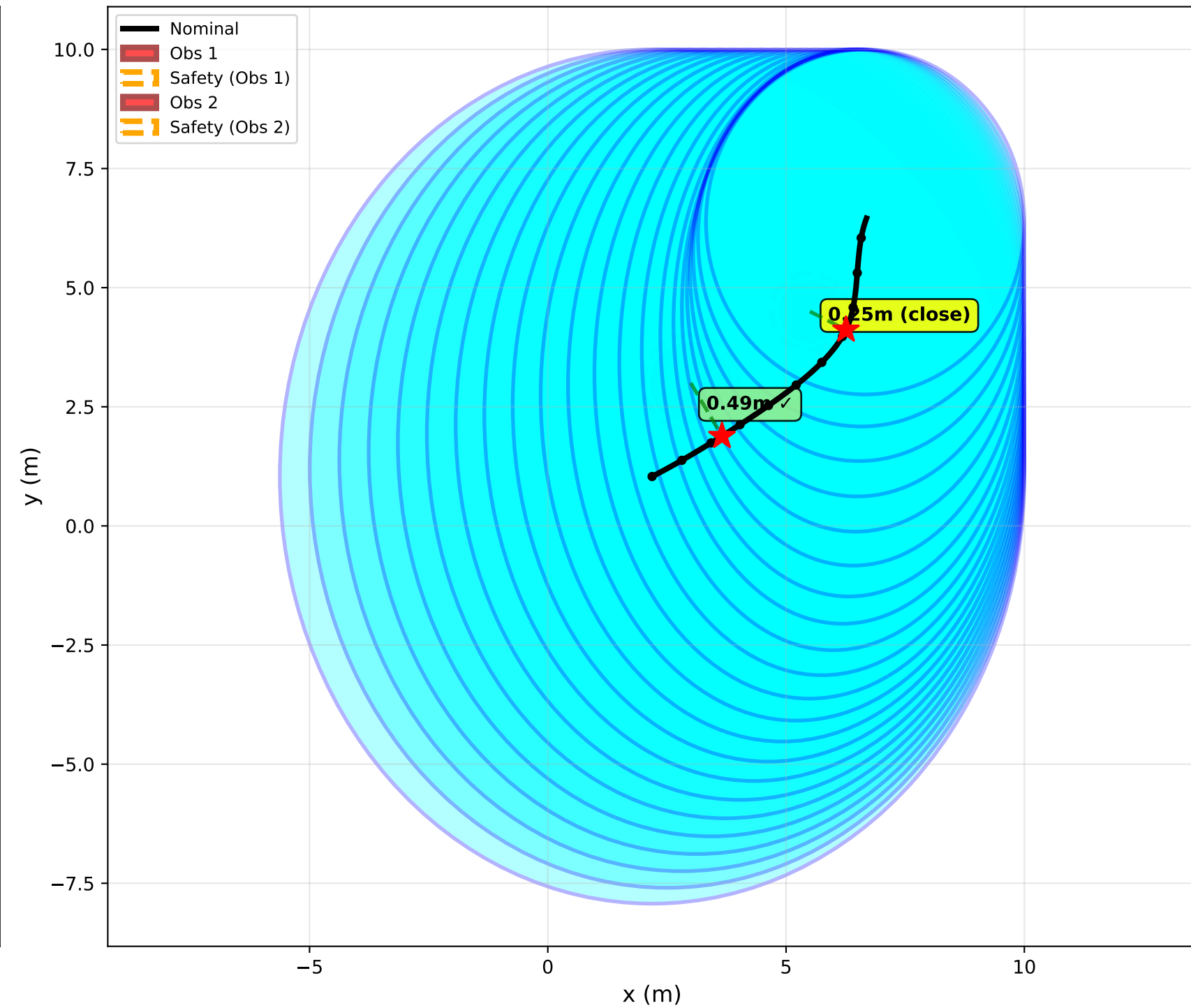
Zoomed: Obstacle Clearance Verification
