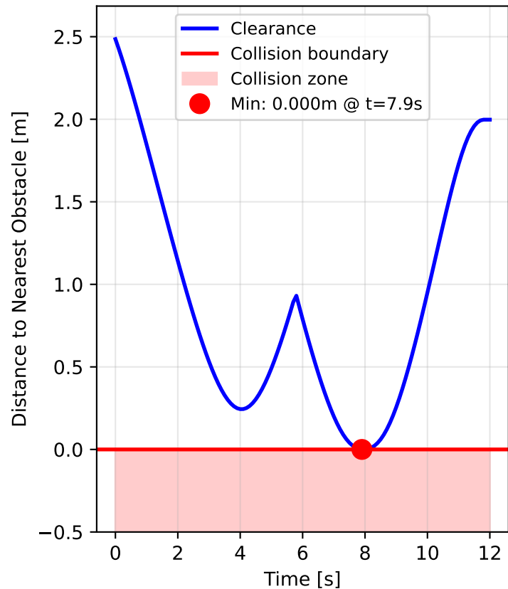
Obstacle Clearance vs Time
