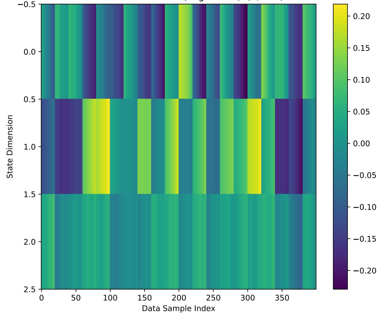
Future State Matrix H+ (Segment 0): (3, 400)
