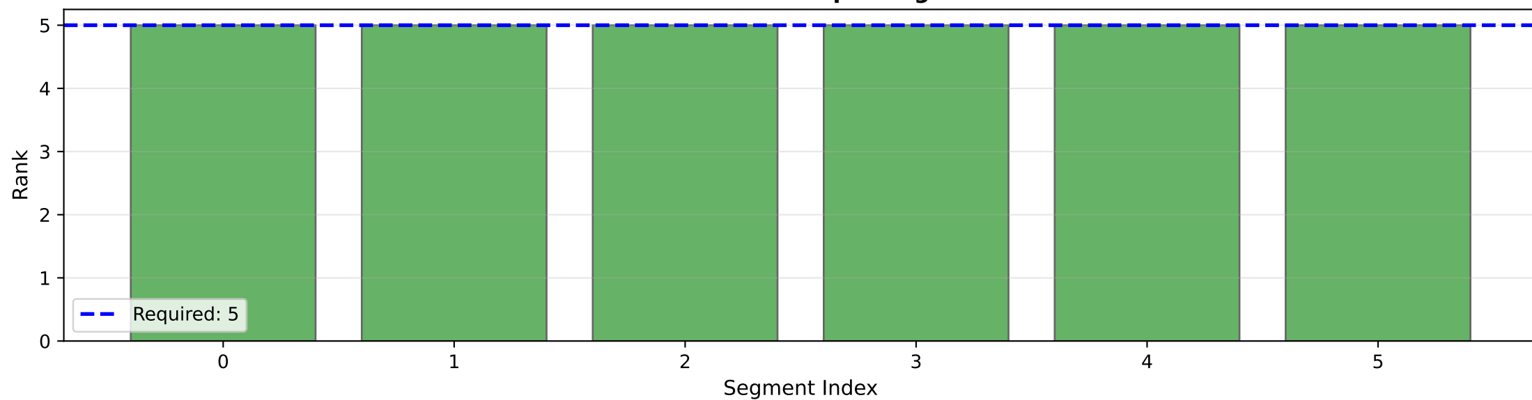
Data Matrix Conditioning
