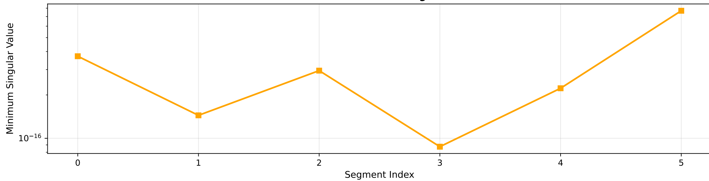
Data Matrix Minimum Singular Value
