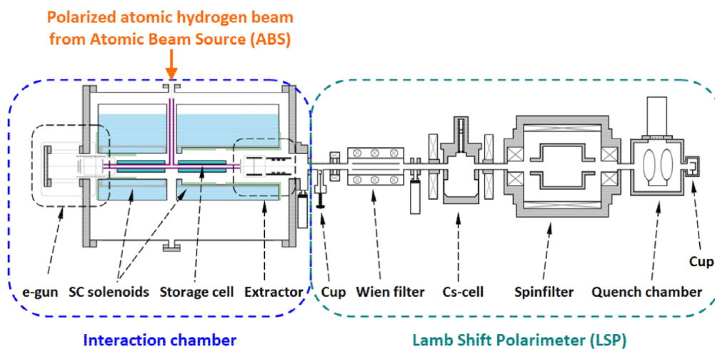
图 2.6.1: The design of the apparatus to produce polarized molecules and to measure their polarization.
