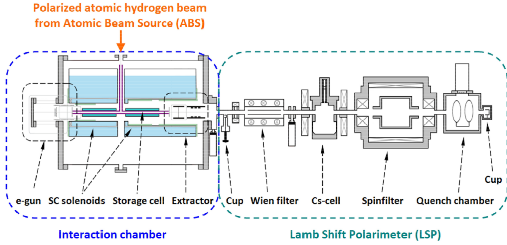
图 4: The design of the apparatus to produce polarized molecules and to measure their polarization.
