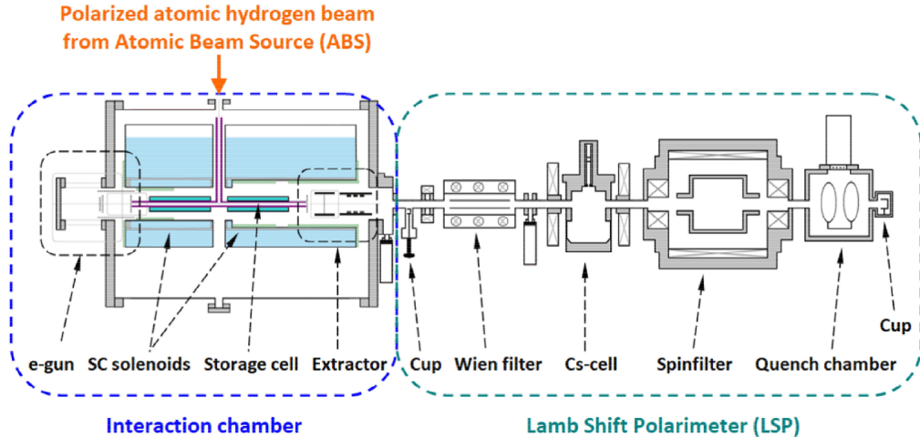
图 4: The design of the apparatus to produce polarized molecules and to measure their polarization.
