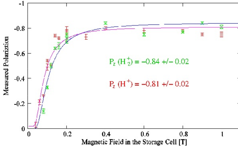
图 5: Measurement of the atomic hydrogen (red) and molecular hydrogen polarization (green) as function of the external magnetic field. At magnetic fields higher than 0.3 T the nuclear polarization of P_z = -0.84 \pm 0.02 is preserved in the molecules.
