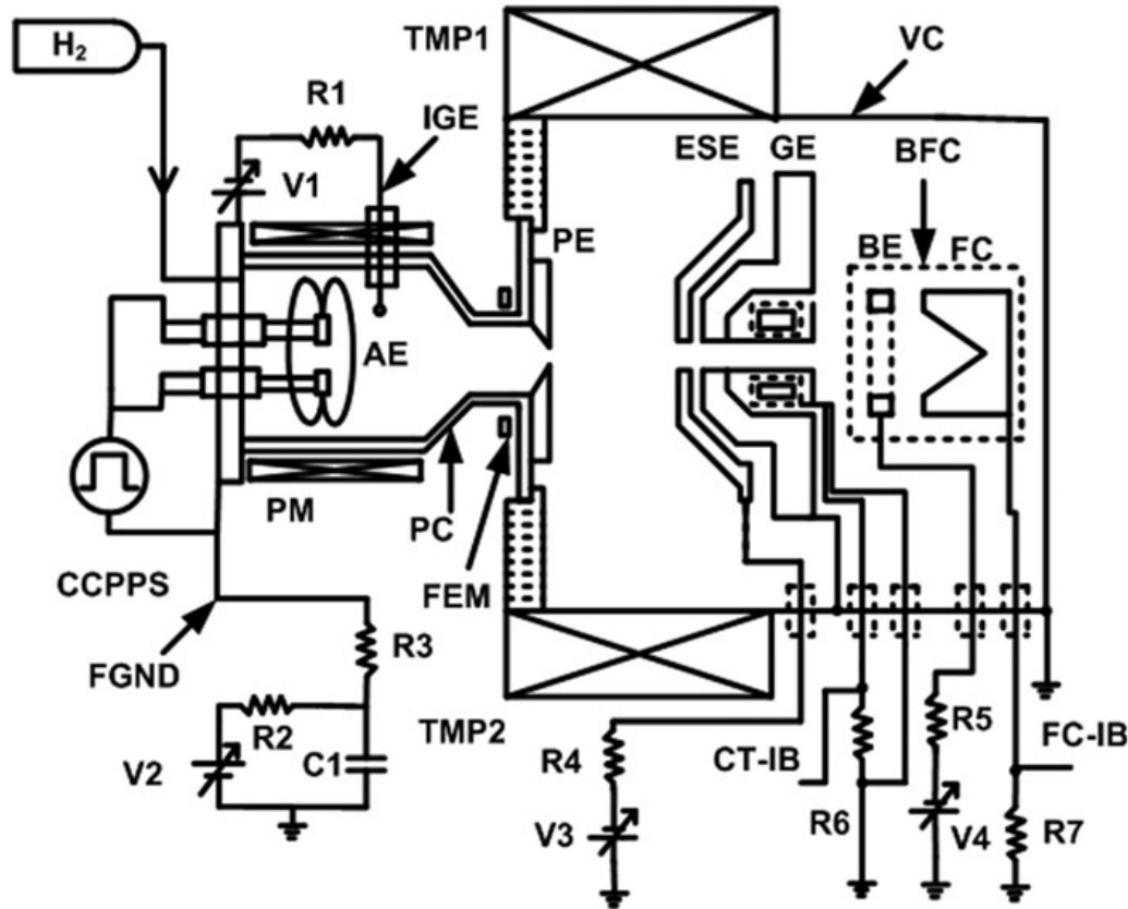
图 1.9.2: 弧放电氢离子源结构: CCPPS: constant current pulsed power supply, FGND: floating ground, IGE: ignition electrode, ESE: electron suppression electrode, TMP: turbomolecular pump, PE: plasma electrode, GE: ground electrode, BFC: biased Faraday cup, FC: Faraday cup, BE: biasing electrode, CT-IB: current transformer positive hydrogen ion current, FC-IB: Faraday cup positive hydrogen ion current, IR: Faraday cup termination resistance, PM: permanent magnet, FEM: filter electromagnet, PC: plasma chamber (cold cathode), AE: arcing electrode (tungsten filament/element), VC: vacuum chamber, V1: ignition power supply, V2: acceleration power supply, V3: electron suppression biasing supply, and V4: Faraday cup biasing electrode power supply.
