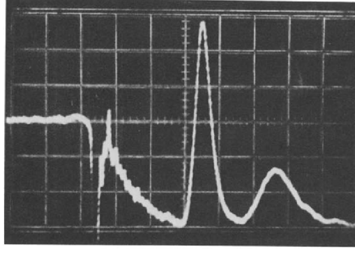
图 1.2.3: Characteristic oscillogram of the mass spectrometer pulses; RF discharge turned on; N = 1 \times 10^{18} molecules per pulse; P_{rf} = 3.6 \text{ kW} , T_{ch} = 300 \text{ K} . From left to right: electron beam current pulse (0.2mA/div), accelerating voltage pulse, and ion current pulses of the atomic and molecular hydrogen (50 mV/div). Horizontal scale: 0.5 \mu\text{s}/\text{div} .
