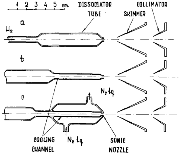
图 1.2.2: Scaled drawing of the dissociator tube and of the system forming the atomic beam.
