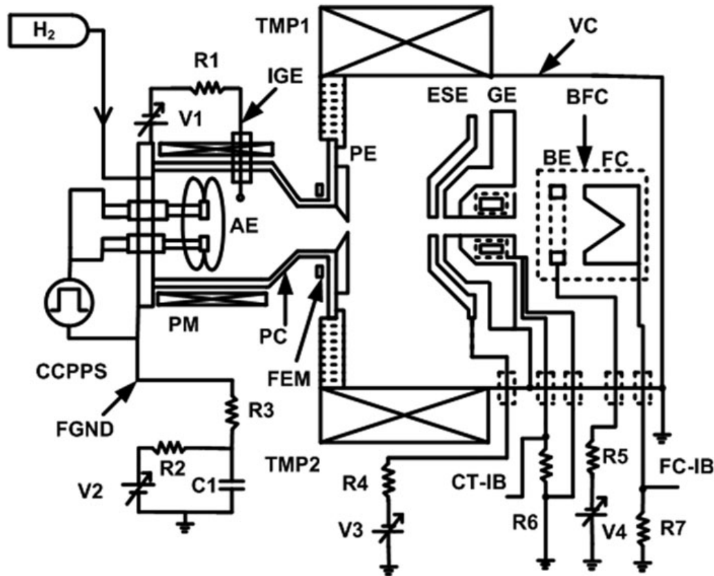
图 1.10.2: 弧放电氢离子源结构: CCPPS: constant current pulsed power supply, FGND: floating ground, IGE: ignition electrode, ESE: electron suppression electrode, TMP: turbomolecular pump, PE: plasma electrode, GE: ground electrode, BFC: biased Faraday cup, FC: Faraday cup, BE: biasing electrode, CT-IB: current transformer positive hydrogen ion current, FC-IB: Faraday cup positive hydrogen ion current, IR: Faraday cup termination resistance, PM: permanent magnet, FEM: filter electromagnet, PC: plasma chamber (cold cathode), AE: arcing electrode (tungsten filament/element), VC: vacuum chamber, V1: ignition power supply, V2: acceleration power supply, V3: electron suppression biasing supply, and V4: Faraday cup biasing electrode power supply.
