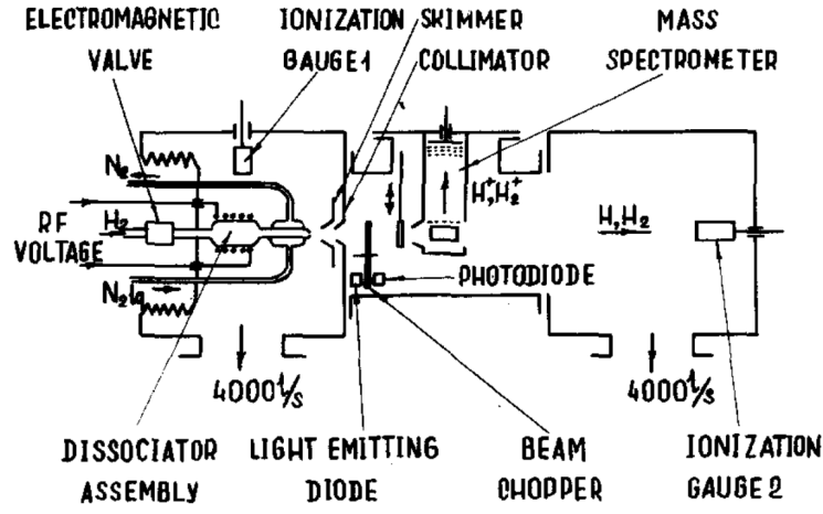
图 1.2.1: Scheme of the experimental set
