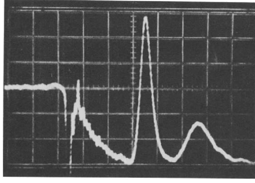
图 1.2.3: Characteristic oscillogram of the mass spectrometer pulses; RF discharge turned on; N = 1 \times 10^{18} molecules per pulse; P_{\text{rf}} = 3.6 \text{ kW} , T_{\text{ch}} = 300 \text{ K} . From left to right: electron beam current pulse (0.2mA/div), accelerating voltage pulse, and ion current pulses of the atomic and molecular hydrogen (50 mV/div). Horizontal scale: 0.5 \mu\text{s}/\text{div} .
