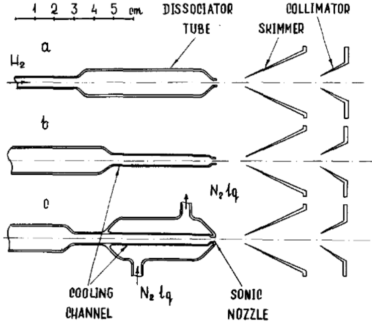
图 1.6.2: Scaled drawing of the dissociator tube and of the system forming the atomic beam.
