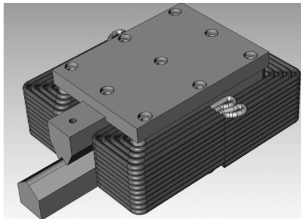
图 1.4.6: CAD drawing of the magnet. The poles are replaceable and slide in a groove on the bottom and top plate for accurate positioning. 40 current carrying copper tubes per coil induce the magnetic field \mathbf{B} .
