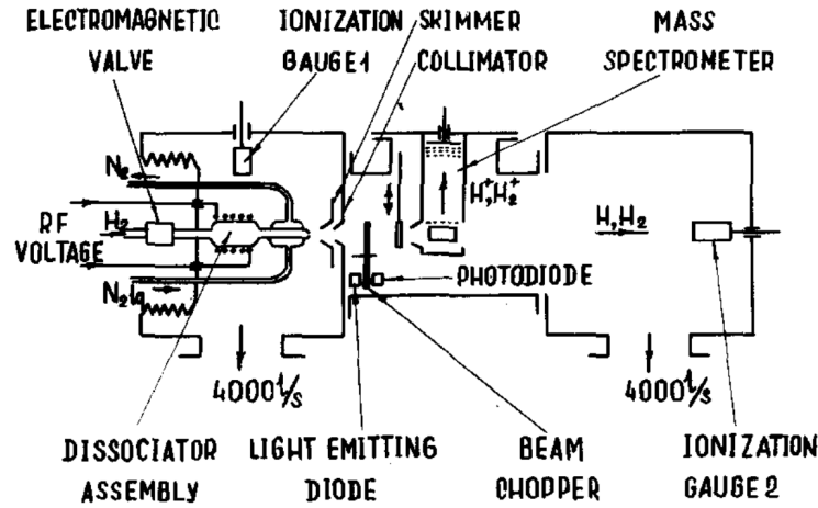
图 1.6.1: Scheme of the experimental set
