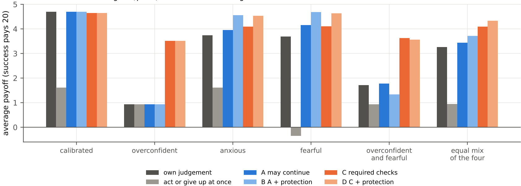
after an overconfident agent ( \gamma = 4 ) hands over: six arrangements
