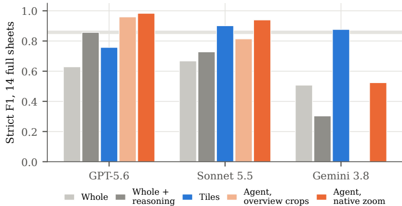
(a) Same model, five ways of using it
