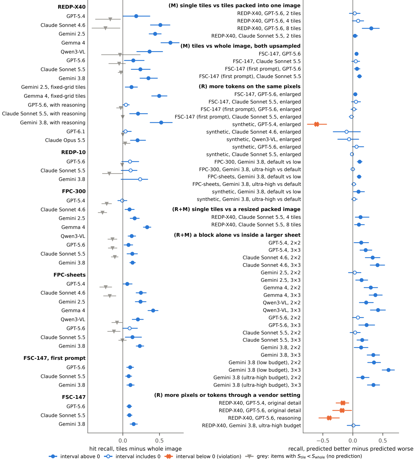
(a) Theorem 1: tiles versus the whole image
