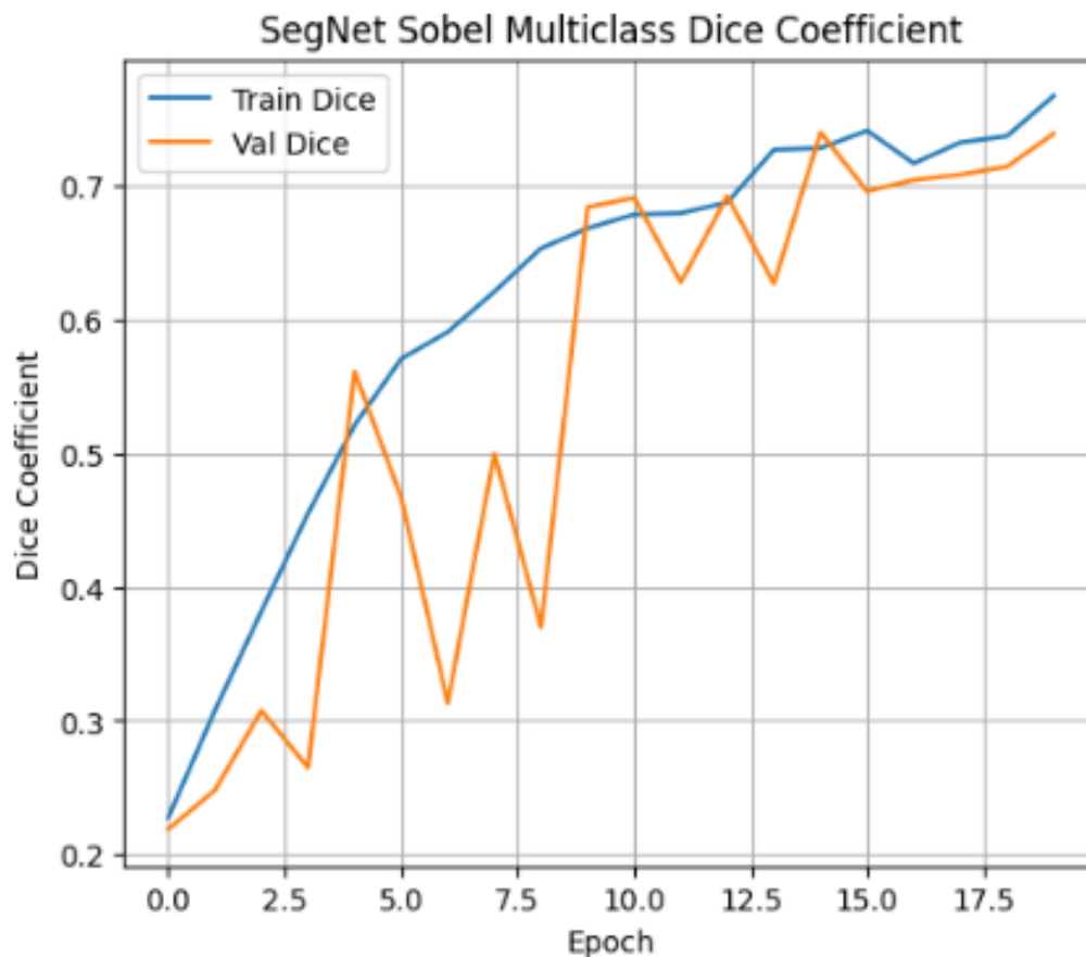
Figure 3.25: Multiclass Dice Coefficient vs. Epoch. Both training and validation curves show steady improvement, with validation Dice exhibiting higher fluctuation due to dataset size and multiclass segmentation complexity.
