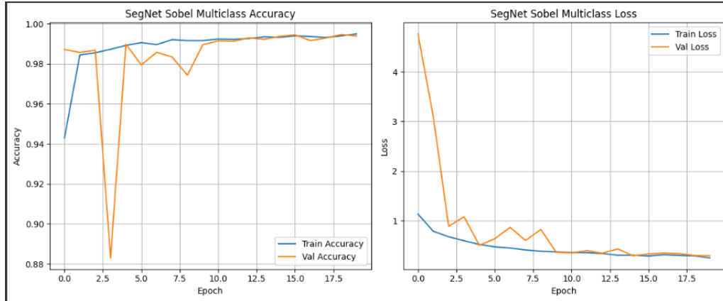
Figure 3.26: Multiclass Accuracy and Loss vs. Epoch. Left: Accuracy improves rapidly to 99% with early validation spikes due to data limitations. Right: Loss decreases sharply and stabilizes, confirming effective learning and generalization.
