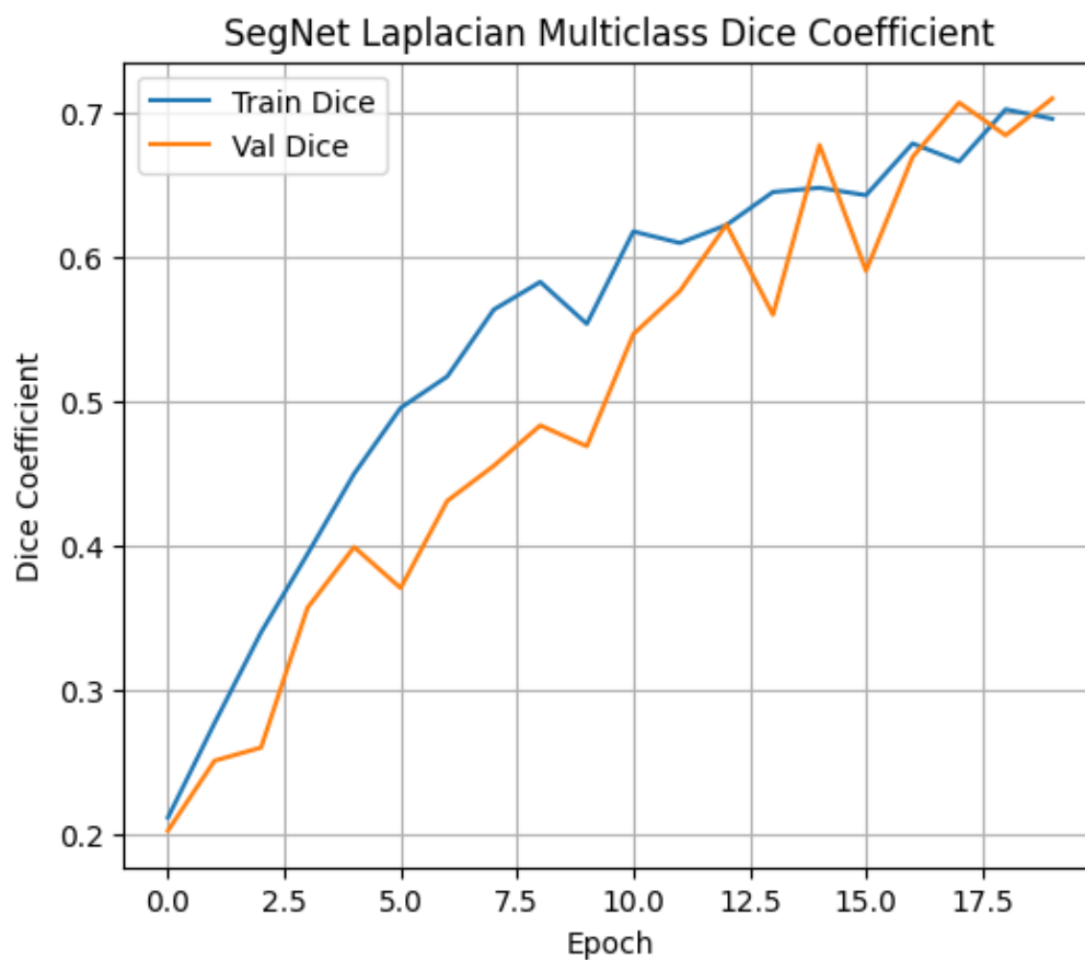
Figure 3.66: Multiclass Dice Coefficient vs. Epoch (Laplacian Filtered) . Validation Dice reaches 0.70+ by final epochs, demonstrating strong Laplacian preprocessing effectiveness.
