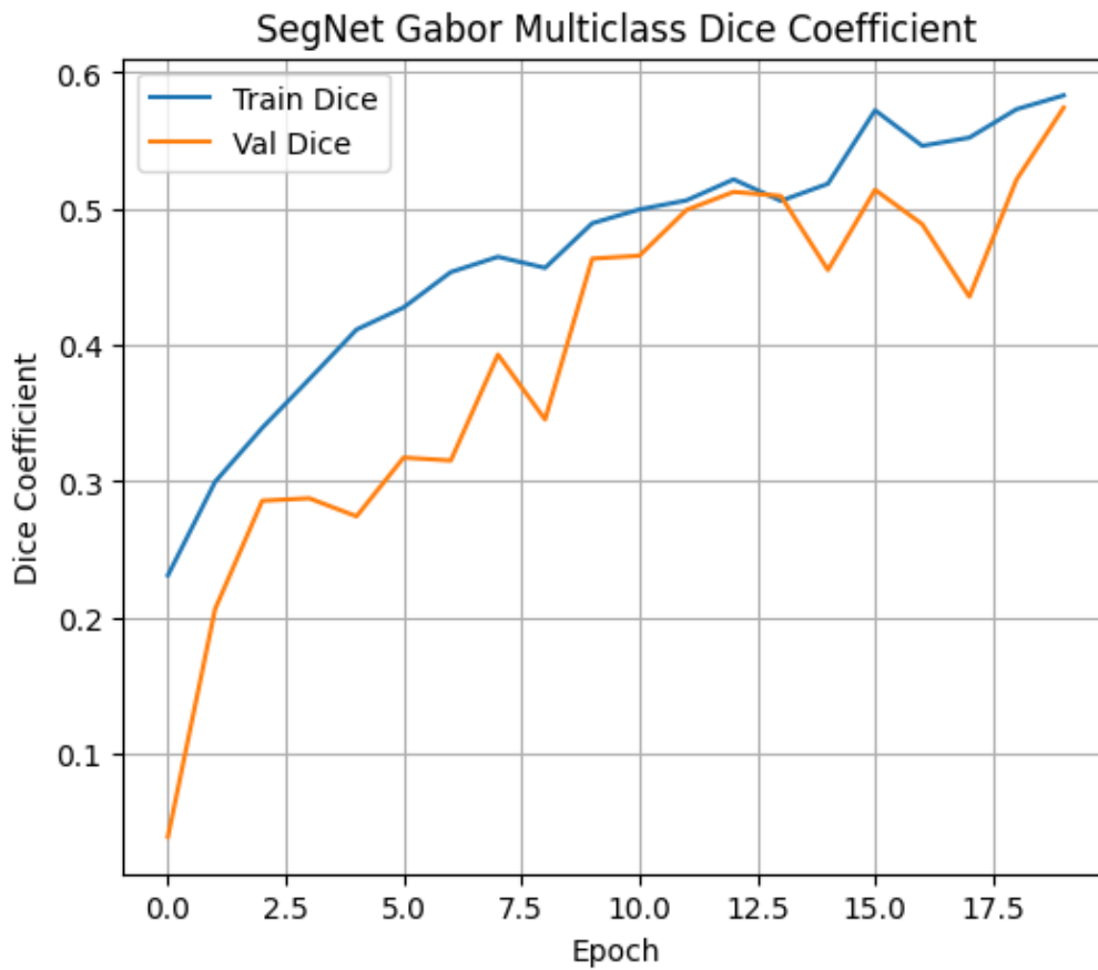
Figure 3.47: Multiclass Dice Coefficient vs. Epoch (Gabor Filtered) . Both training and validation curves show steady improvement, with validation Dice exhibiting higher fluctuations due to dataset size and segmentation complexity.
