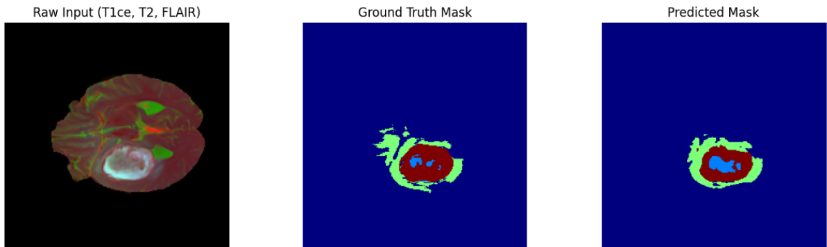
Figure 3.96: Raw Input, Ground Truth, and Predicted Mask – Example 4.
