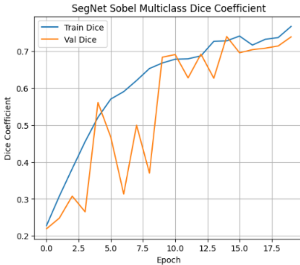
Figure 3.25: Multiclass Dice Coefficient vs. Epoch. Both training and validation curves show steady improvement, with validation Dice exhibiting higher fluctuation due to dataset size and multiclass segmentation complexity.
