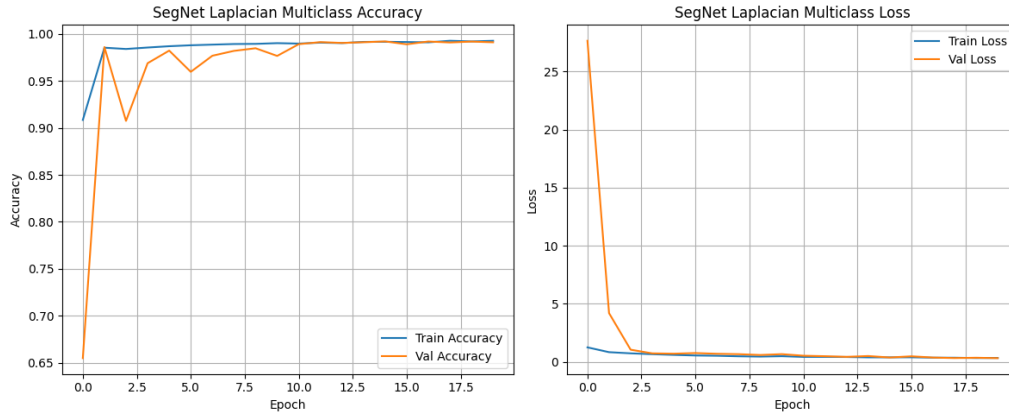
Figure 3.67: Accuracy & Loss vs. Epoch (Laplacian). Rapid convergence with accuracy plateauing at 99% and loss stabilizing at low values.
