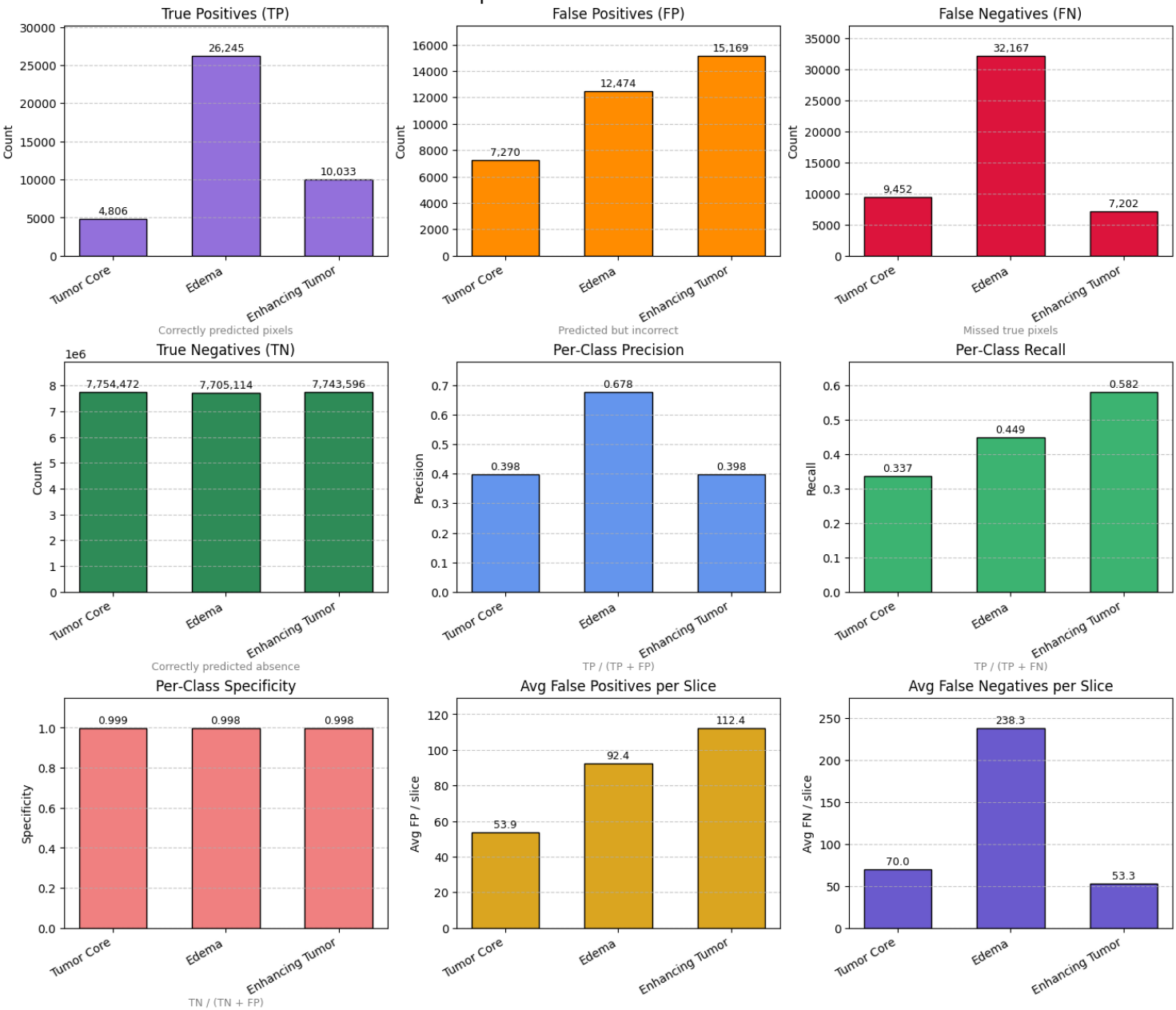
Gabor-Pipeline Per-Class Pixel Metrics
