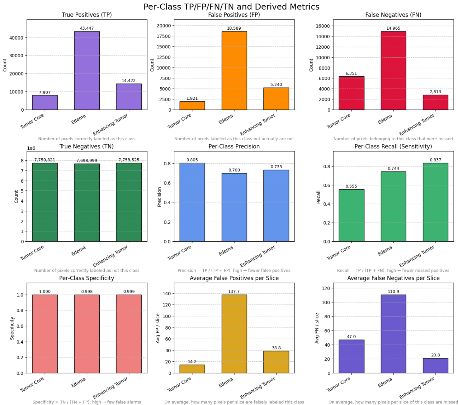
Figure 3.8: Visualization of per-class pixel-level metrics (TP, FP, FN, TN, precision, recall, specificity, average FP/FN per slice) for the no-preprocessing pipeline.
