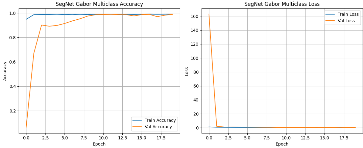
Figure 3.48: Multiclass Accuracy and Loss vs. Epoch (Gabor Filtered). Left: Accuracy improves rapidly to near-perfect values with occasional fluctuations. Right: Loss decreases sharply, confirming effective learning on Gabor-filtered data.
