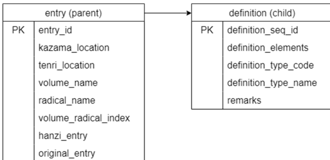
ER_notes diagram
