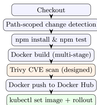
Figure 18: Per-service Jenkins pipeline stages. Orange stage is the DevSecOps gate.
