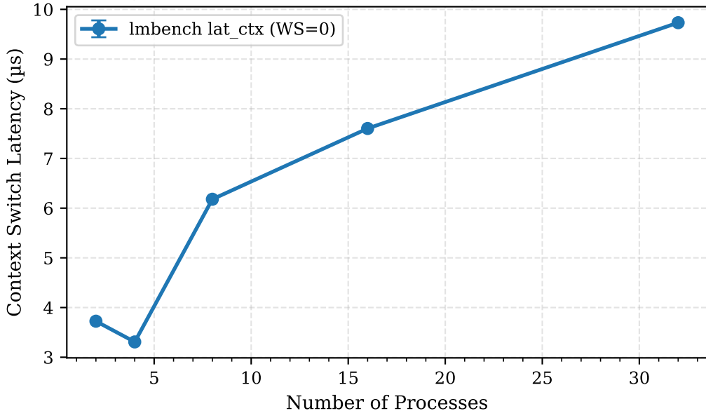
Fig 1: Scheduler Scaling — Latency vs Process Count
