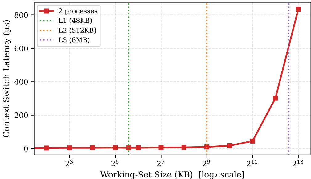
Fig 2: Working-Set Effect on Context-Switch Latency (lmbench)
