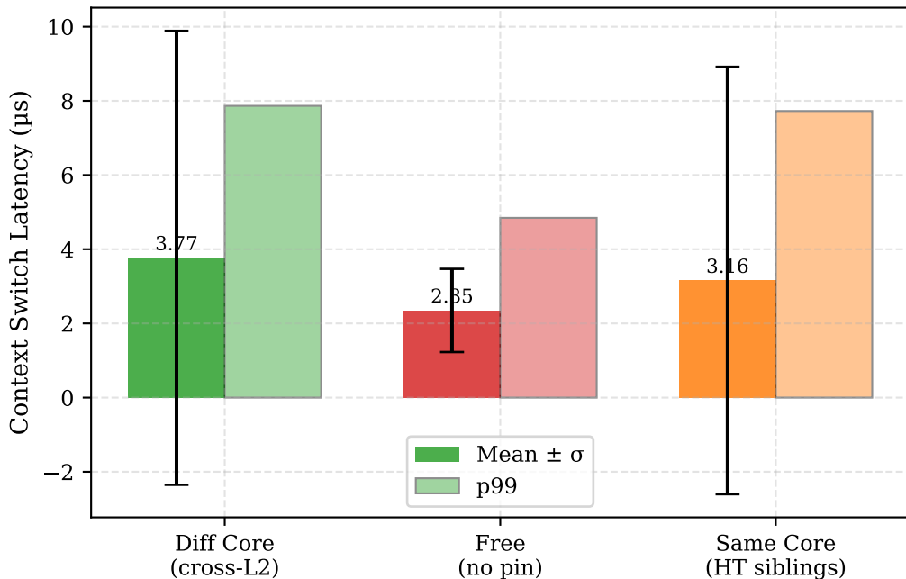
Fig 3: Core Migration Penalty — Same vs Cross Core
