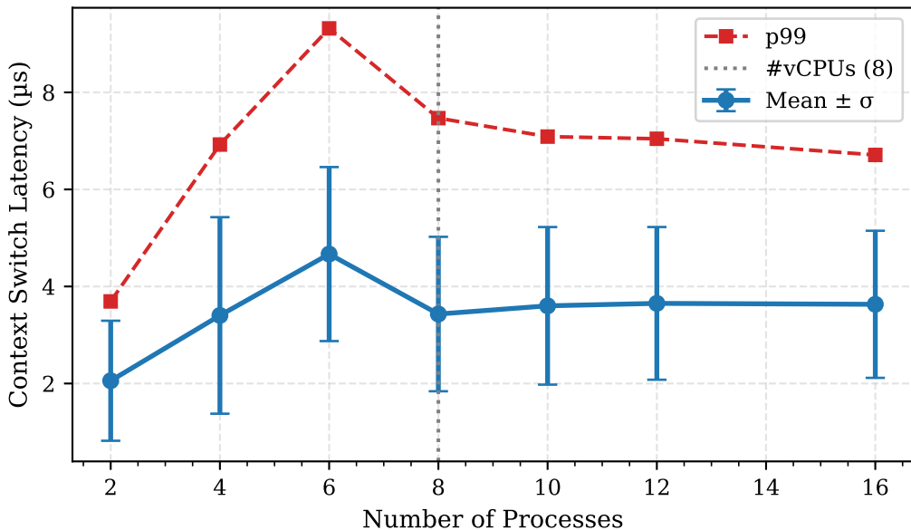
Fig 4: Scaling Analysis — Latency vs Process Count
