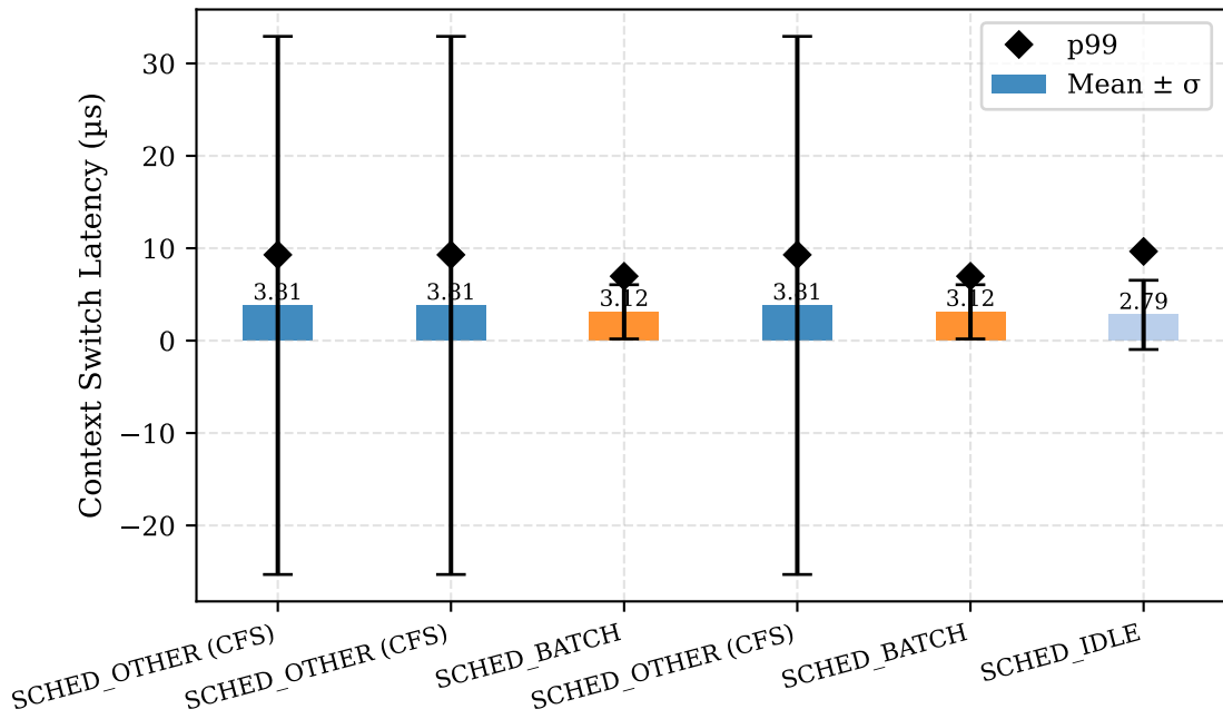
Fig 5: Scheduler Policy Comparison
