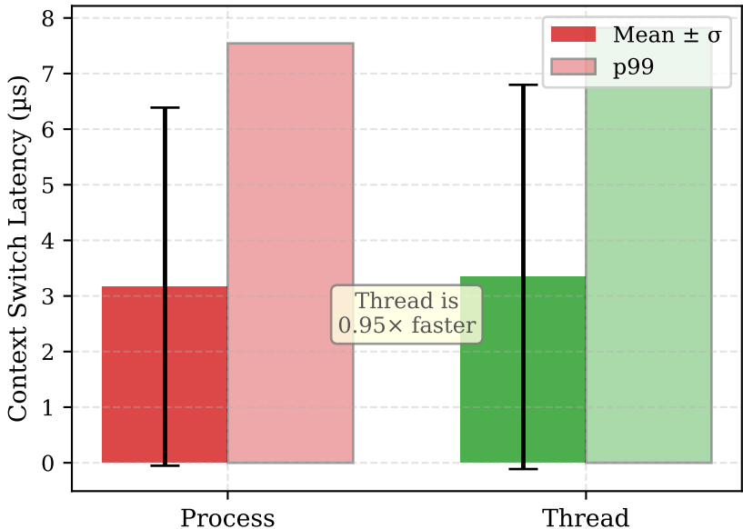
Fig 6: Process vs Thread Context Switch
