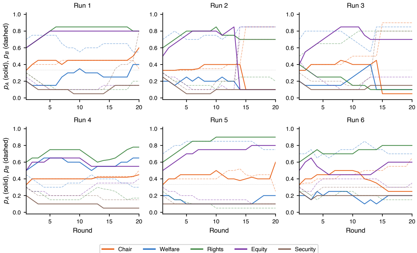
Per-agent preferences ( p_A solid, p_B dashed) — IM-01, T = 0 , roles=True; 6 representative runs
