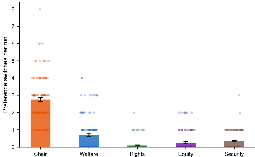
Per-agent switch counts by role (IM-01, T \in \{0, 0.01, 0.05, 0.1, 0.2, 0.7\} , roles=True; 600 agent-runs)
