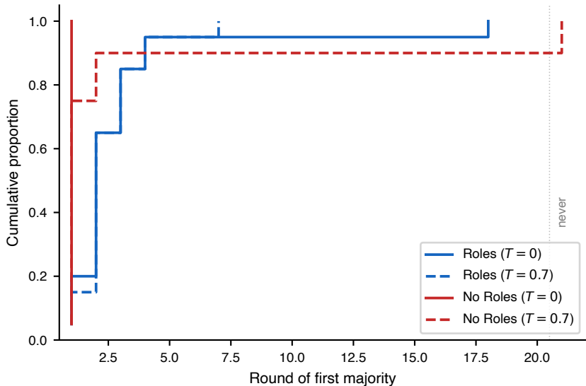
Time-to-majority: ECDF across replicates (IM-01)
