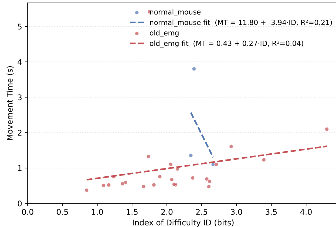
Fitts' law: movement time vs. index of difficulty
