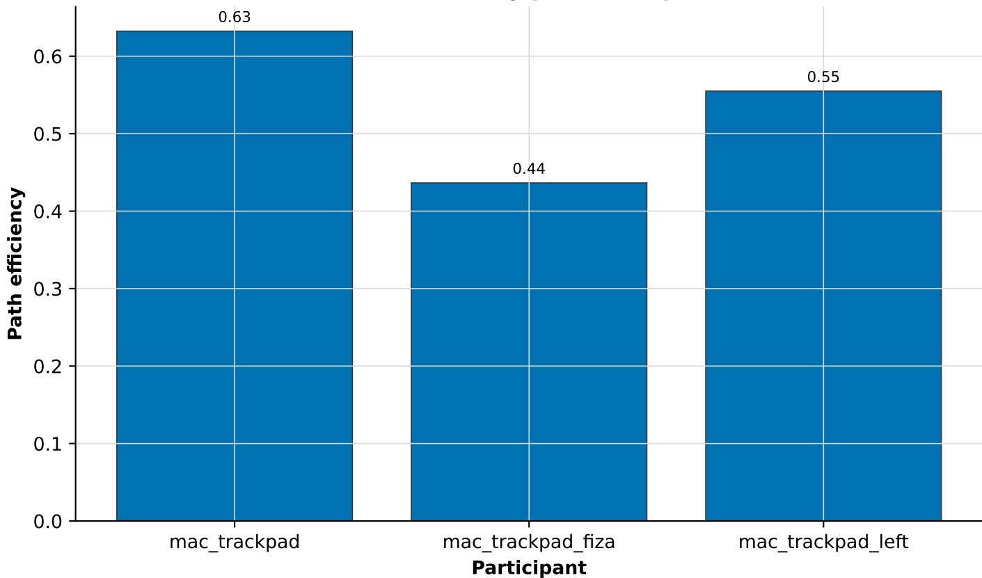
Path Efficiency per Participant
