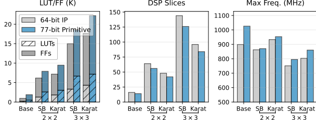
Figure 7: Resource and frequency comparison between the 64-bit AMD IP and our 77-bit base multiplier when tiled to larger sizes.
