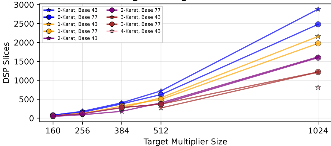
DSP Usage vs Target Size (Line Plot)
