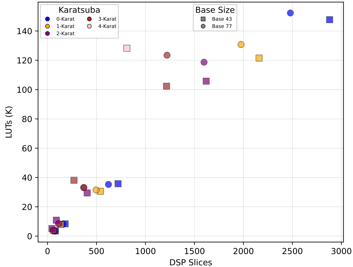
DSPs vs LUTs
