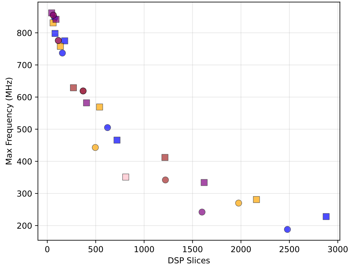
DSPs vs Frequency
