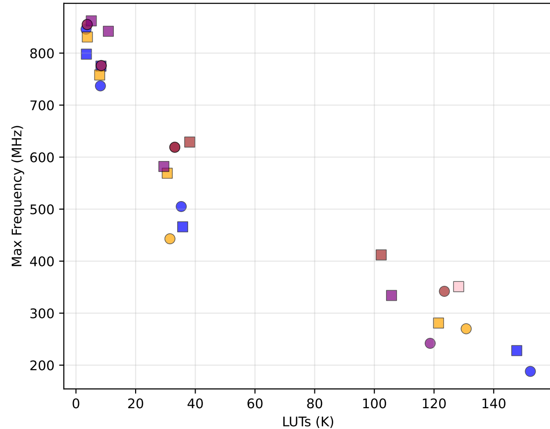
LUTs vs Frequency
