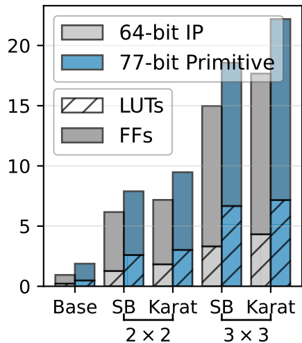
LUT/FF (K)
