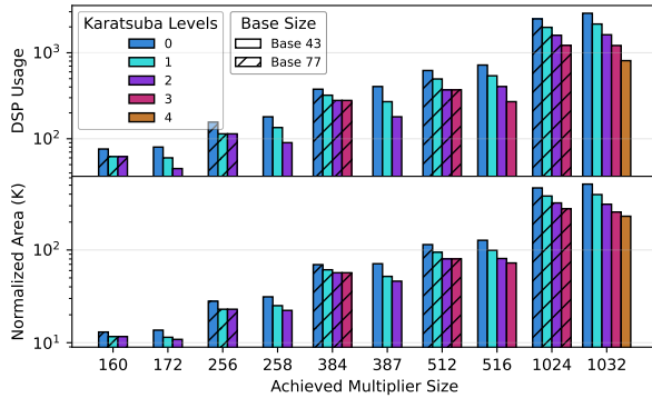
Fig. 9: Resource utilization for target-constrained tiling using our 77-bit base and overshoot tiling using our 43-bit base multipliers, with varying numbers of Karatsuba levels. 77-bit base is favorable for fewer Karatsuba levels, while 43-bit base benefits from deeper Karatsuba hierarchies. Note the logarithmic y-axis.
