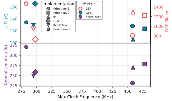
Fig. 10: Area and Performance comparison of different implementations. Our primitive-based implementation achieves approximately 56% higher frequency than the best among other work while using 17% fewer DSPs and slightly fewer LUTs.
