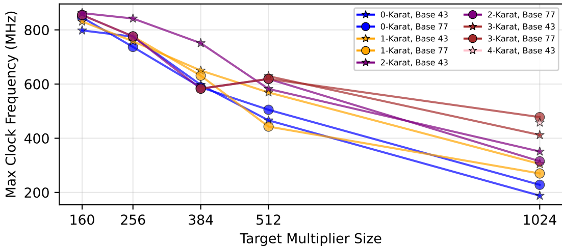
Frequency vs Target Size (Line Plot)
