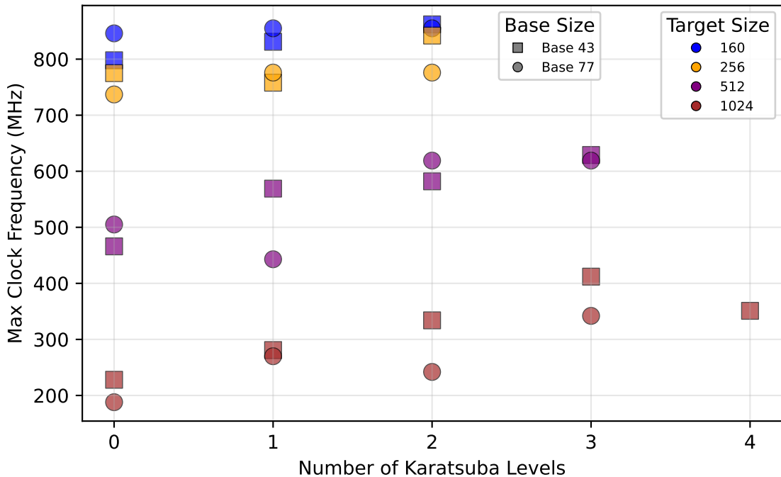
Frequency by Karatsuba Levels
