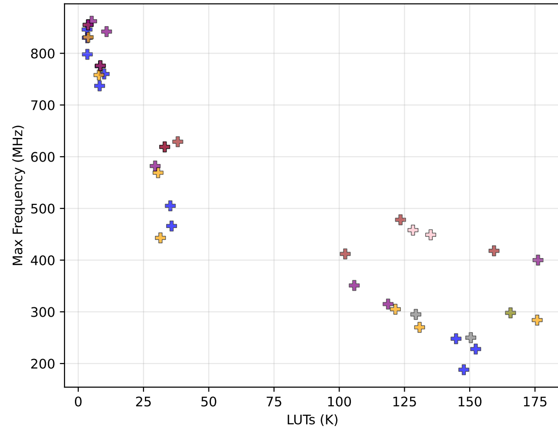
LUTs vs Frequency
