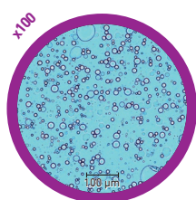
Dispersion without Emulfree® CBG MB
