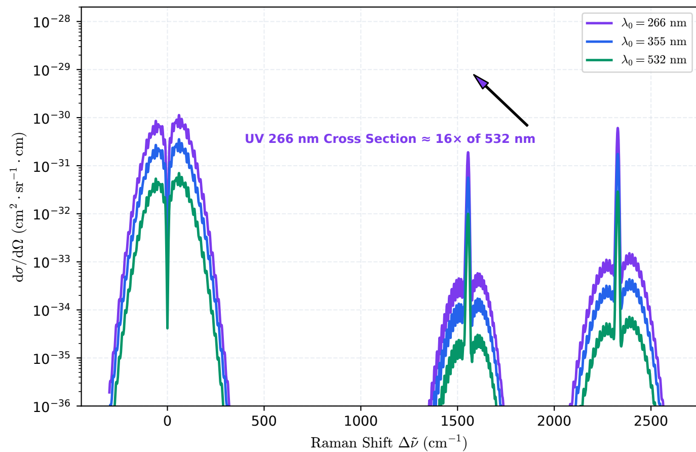
(a) Multi-Wavelength Excitation Dispersion [(\nu_0 - \Delta\nu)^4 \text{ Scaling}]
