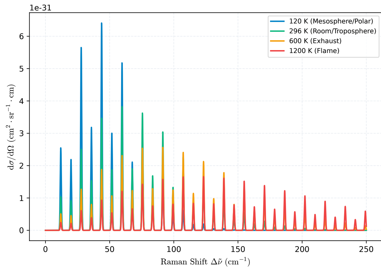
(c) Temperature Dependence of \text{N}_2 Pure Rotational Envelope
