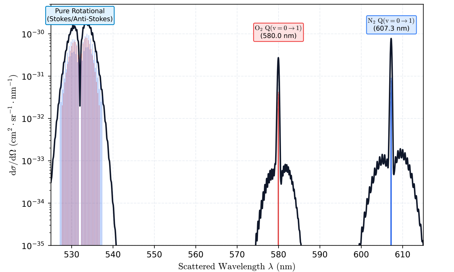
(b) Standard Air Raman Spectrum ( \lambda_0 = 532 \text{ nm} , T = 296 \text{ K} )
