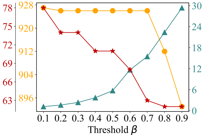
(b) TensorFlow
