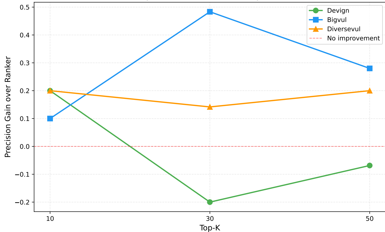
LLM Top-K Candidate Precision Improvement
