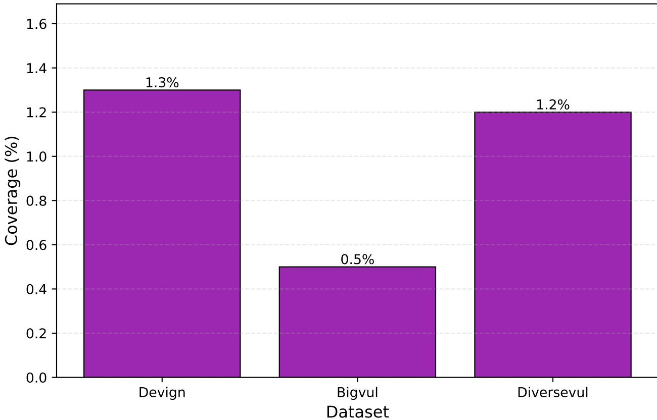
CodeQL Static Analysis Coverage (Function-Level Evaluation)
