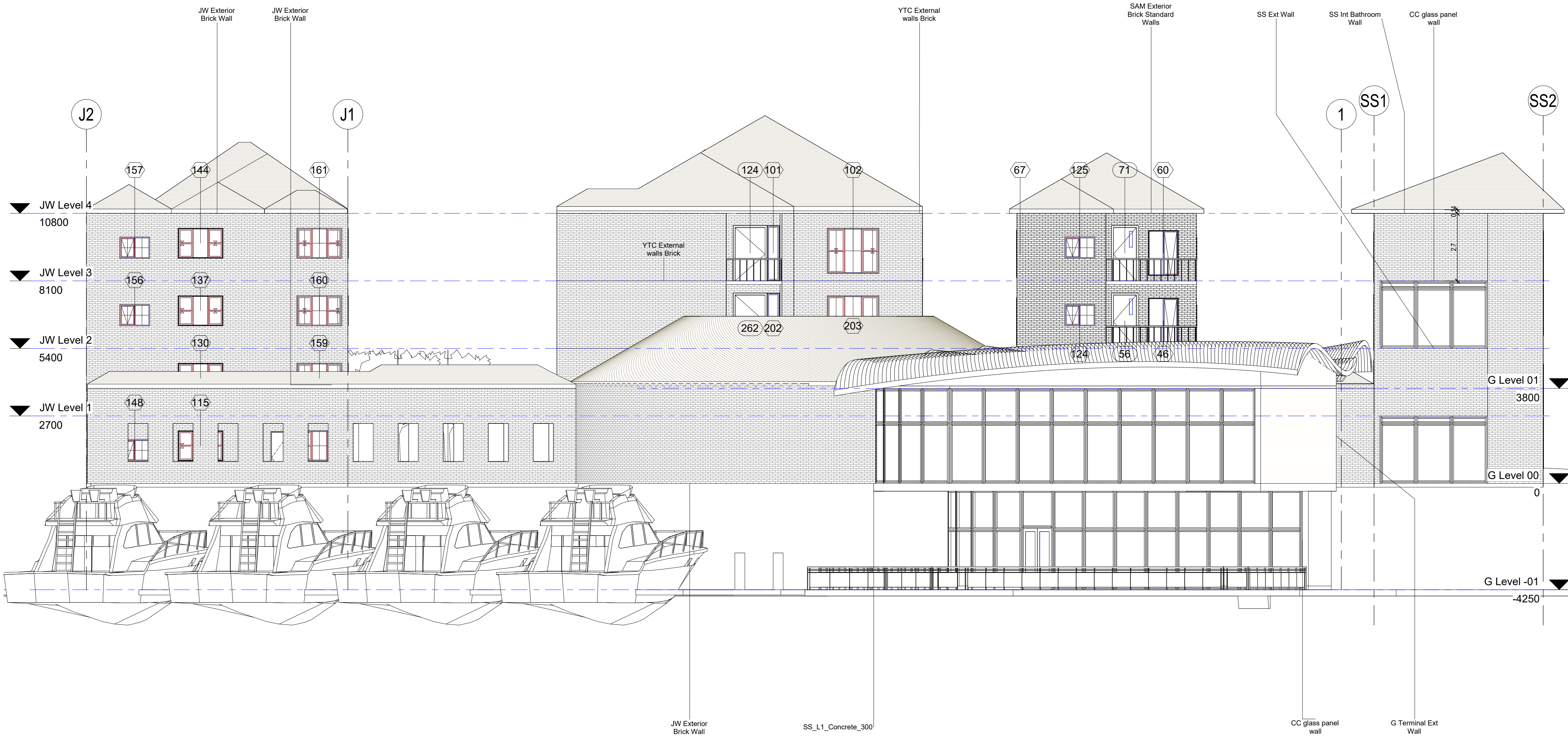
1 HC West Elevation 1 : 100
