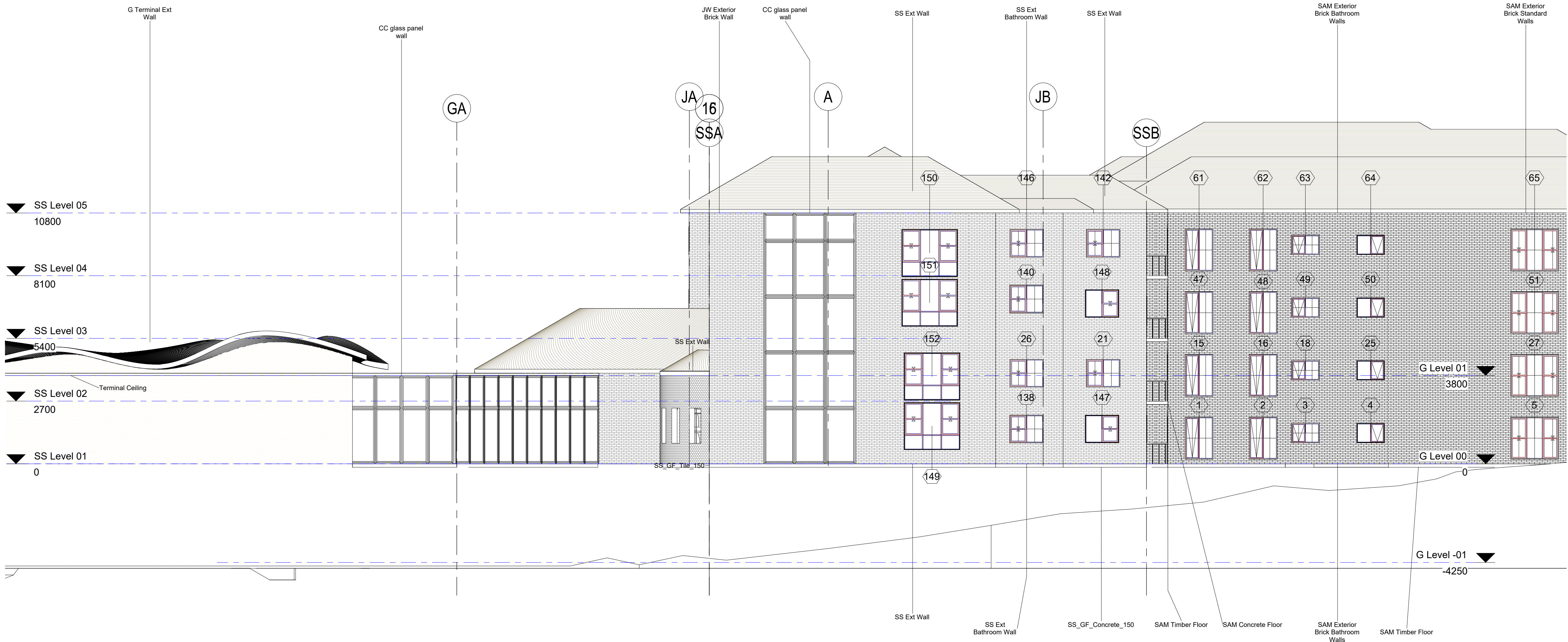
1 HC South Elevation 1 : 100
