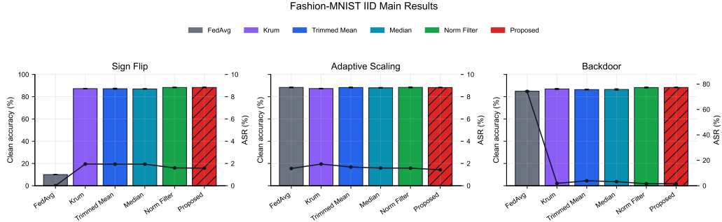
Figure 1: Clean accuracy and attack success rate on Fashion-MNIST under IID data. Bars report mean clean accuracy over three seeds, error bars report standard deviation, and the line reports ASR.
