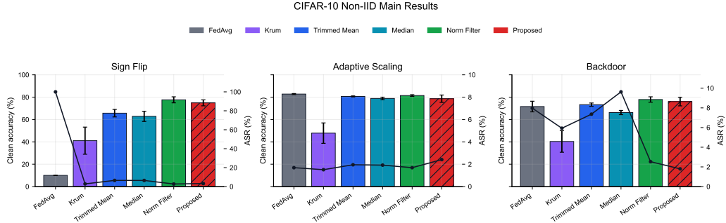
Figure 3: Clean accuracy and attack success rate on CIFAR-10 under Dirichlet Non-IID data. Norm filtering achieves the highest clean accuracy in most settings, while the proposed method remains competitive and maintains low ASR with auditable aggregation decisions.
