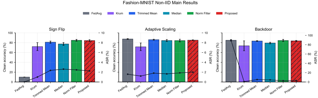
Figure 2: Clean accuracy and attack success rate on Fashion-MNIST under Dirichlet Non-IID data. FedAvg collapses under sign-flip attacks and shows high ASR under backdoor attacks, while robust aggregation methods maintain competitive clean accuracy and suppress ASR.
