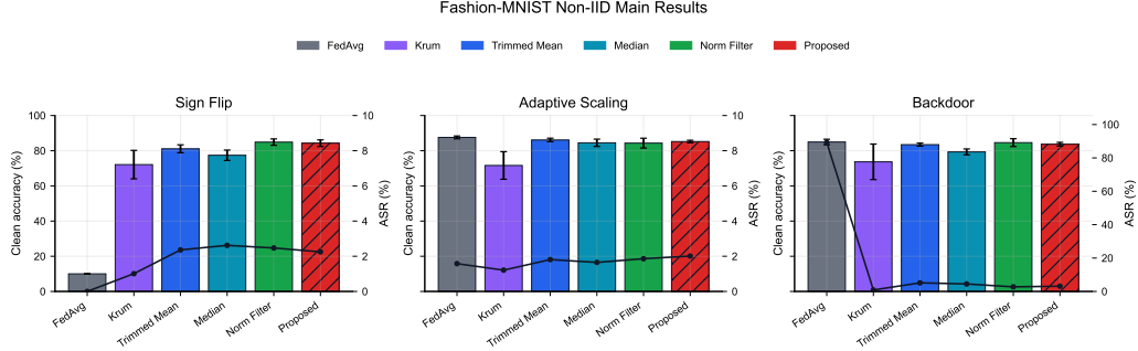
Figure 3: Fashion-MNIST Dirichlet Non-IID results. Bars show three-seed mean clean accuracy with standard-deviation error bars; the line shows ASR. Higher accuracy and lower ASR are better.
