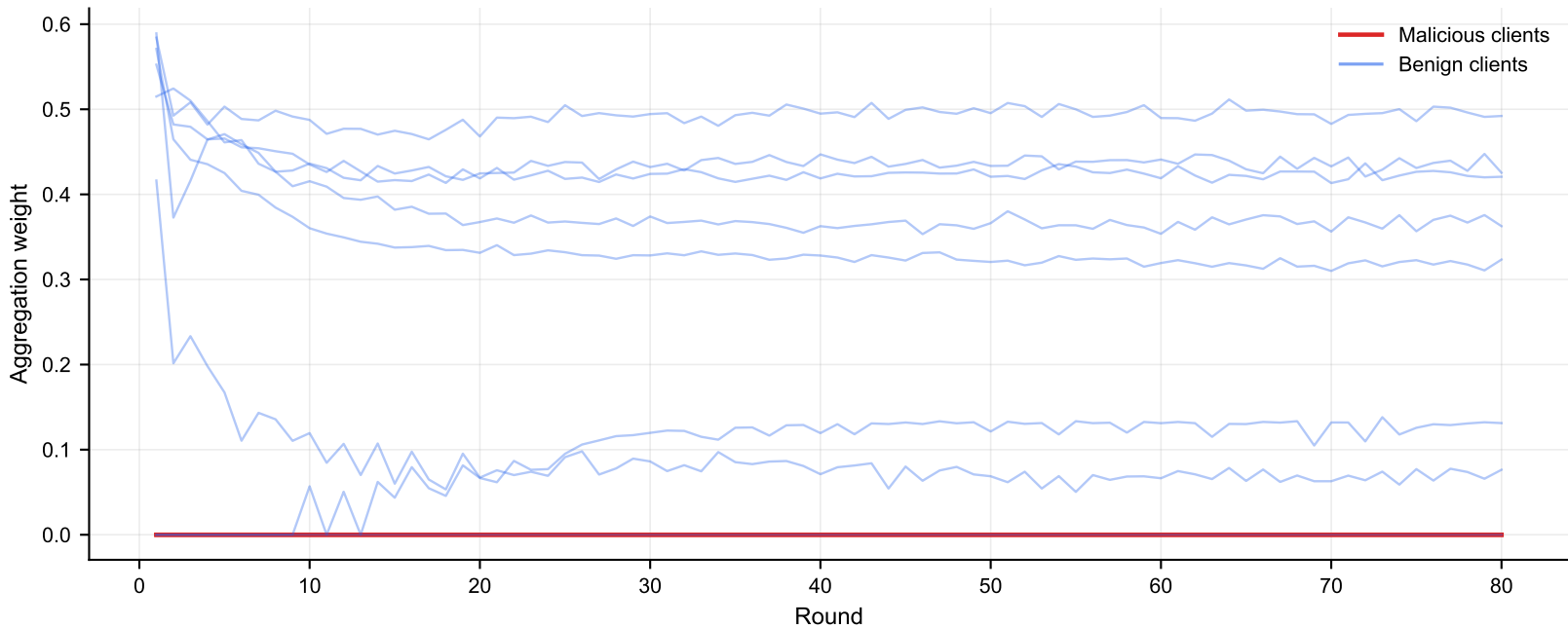
Per-Client Aggregation Weights
