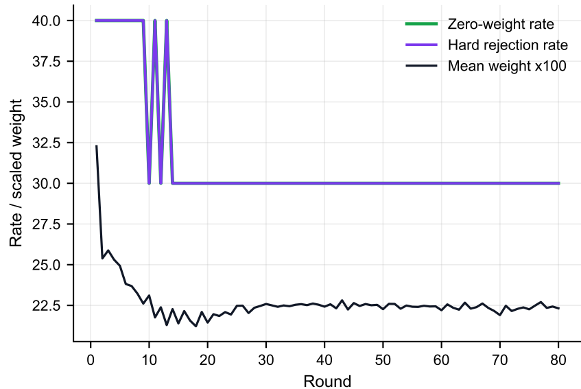
Aggregation Decisions
